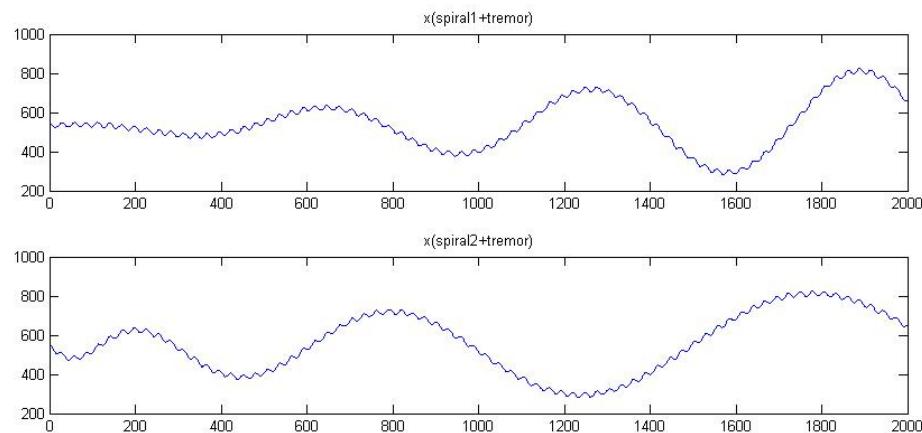
Figure III.3.1 Value of x coordinates through time (coordinate vs tp ). The figure in the upper frame is x(n) of tremor1, the figure in the lower frame is x(n) of tremor2. y(n) of both tremor1 and tremor2 are the same as its component spiral, as shown in Chapter II.
